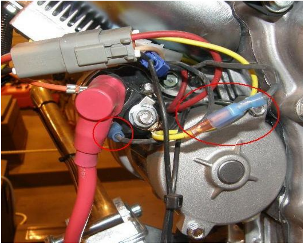
Briggs & Stratton 35hp Mercury Switch Wire Connections
